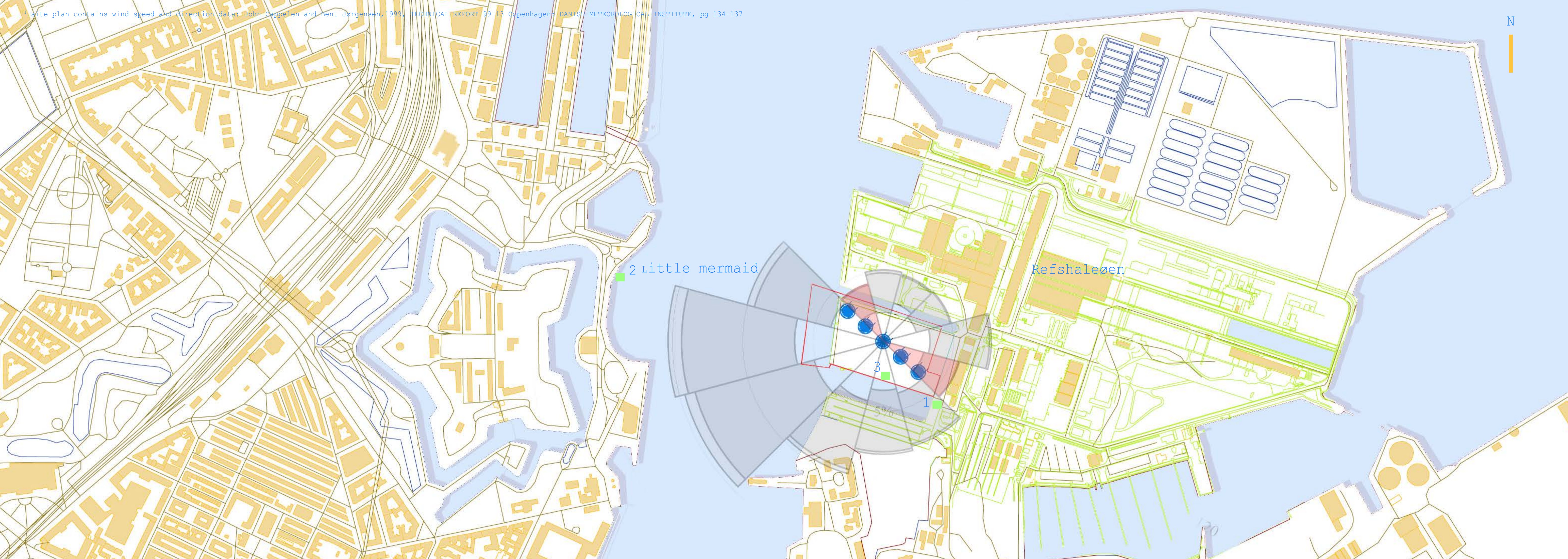
Site Plan Site boundaries in red, blue circles indicate the locations of the wind turbines. They are placed in such a way so as to minimise loss. Wind statistics taken from Copenhagen airport 8.7km away, the red sectors indicate the wind not taken into calculations due to tower blockage and unit alignment.
