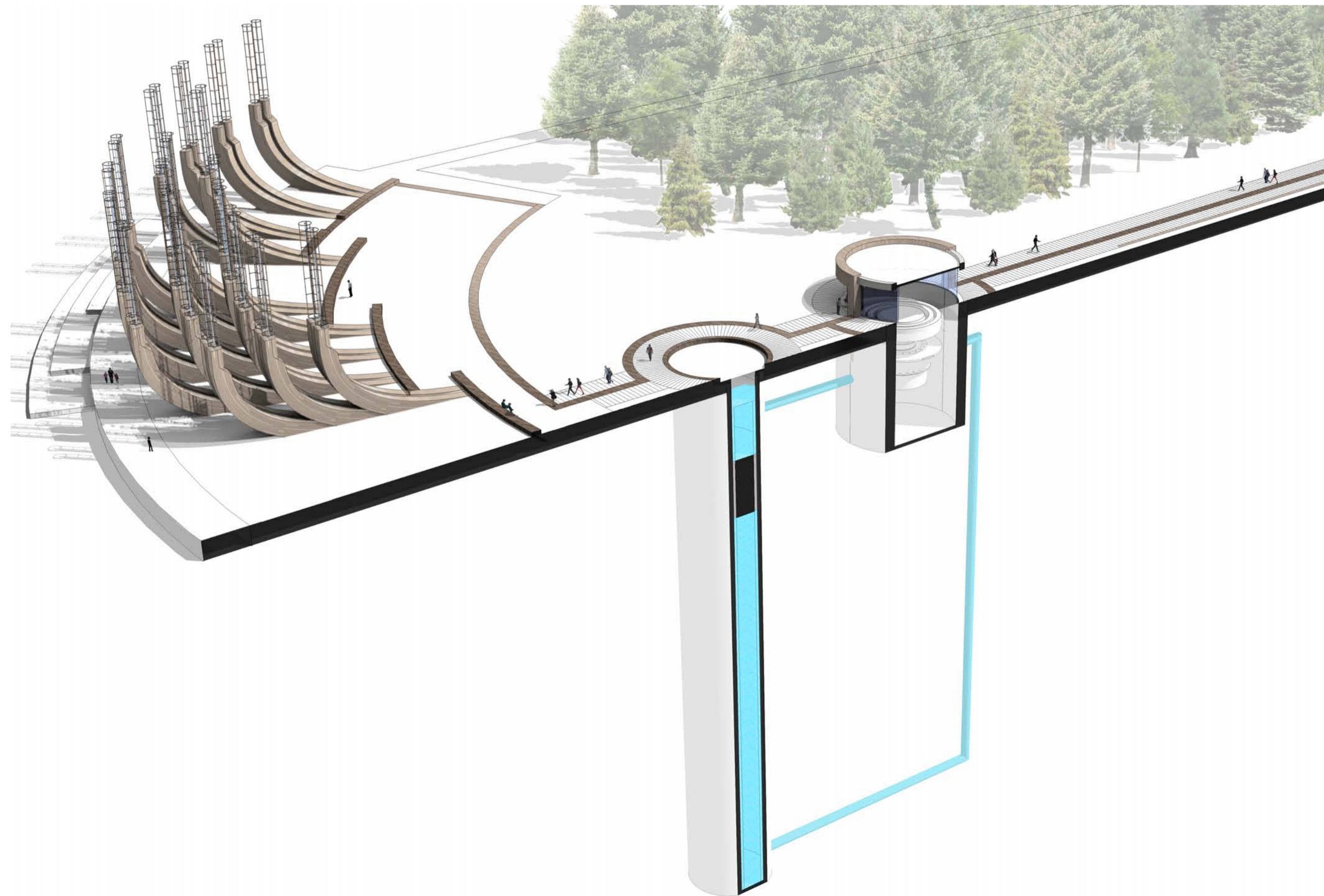
CUT-AWAY VIEW OF GRAVITY STORAGE SYSTEM
